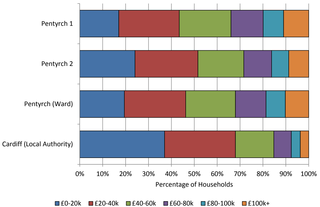
Household Income by Income Band (Pentyrch), 2015
